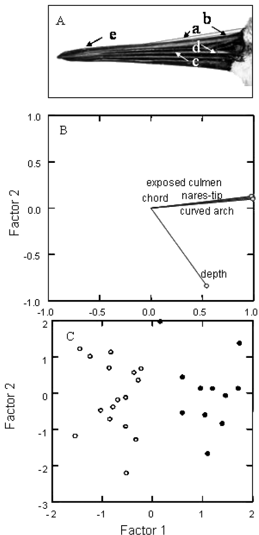
Figure 1. A. Five dimensions of Western Sandpiper bill shape (see Methods for details). B. Bill length and related variables constituted Factor 1, which explained 84% of the variance in bill shape. Bill depth constituted Factor 2. C. Males (open circles) and females (filled circles) differed only with regard to Factor 1 (bill length), but not Factor 2 (bill depth).
